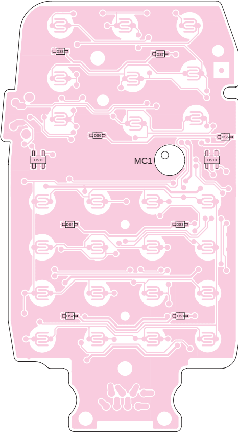
8-1 HM-133V • TOP VIEW
